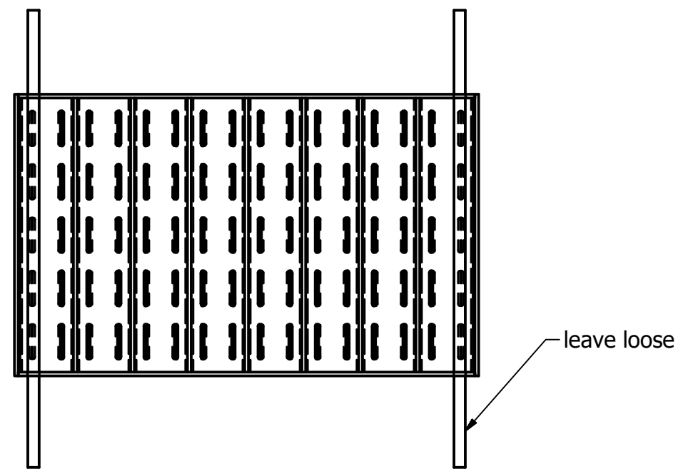
Grate Detail
