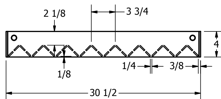
Grate Detail
