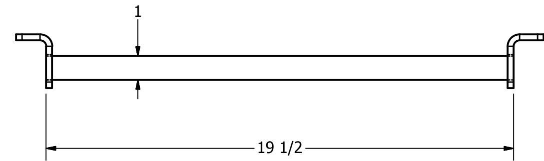
Grill Detail
